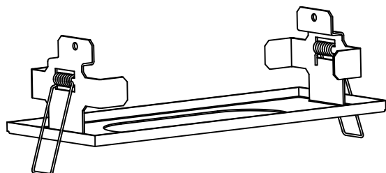
Masking frame with springs
